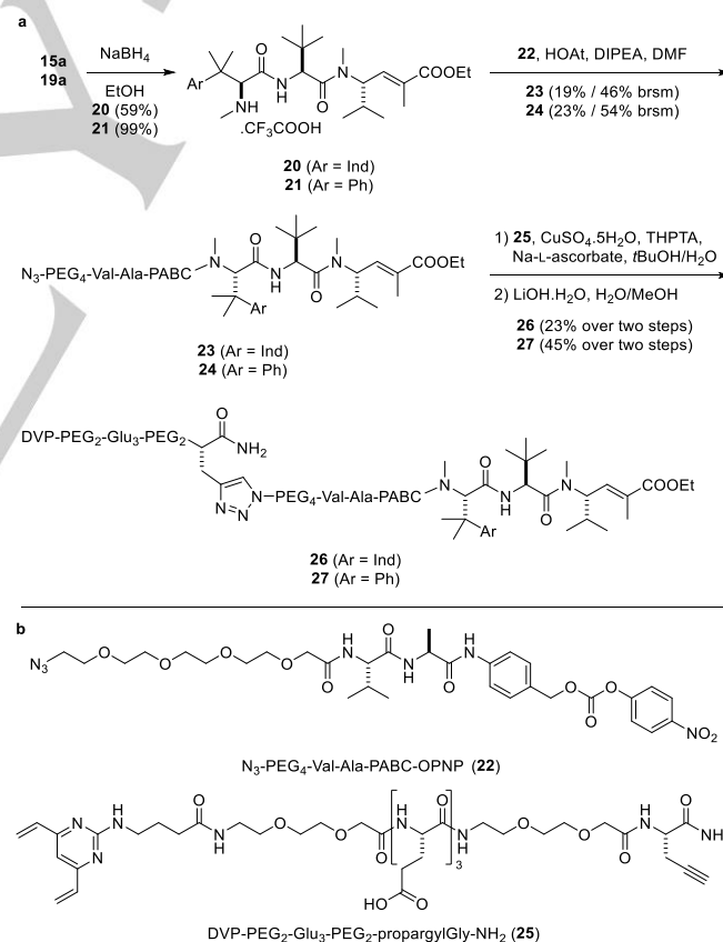
Scheme 4 a) Synthesis of linker-drug compounds 26 and 27 . b) Structures of 22 and 25 (see SI for the syntheses). PABC = p -aminobenzoyloxycarbonyl, HOAt = 1-hydroxy-7-benzotriazole, THPTA = tris(3-hydroxypropyl)triazolyl(methyl)amine
