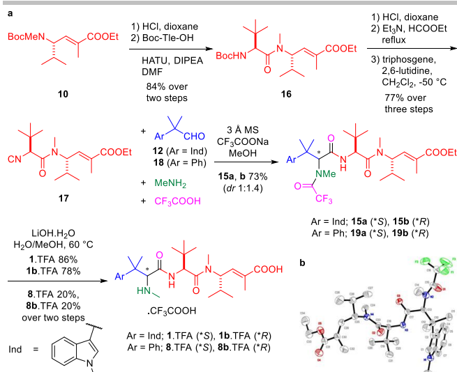
Scheme 3 a) Final route to the synthesis of hemiasterlin ( 1 ) and taltobulin ( 8 ). b) X-ray crystal structure of intermediate 15a . [50] HATU = hexafluorophosphate azabenzotriazole tetramethyl uronium, DIPEA = diisopropylethylamine, TFA = trifluoroacetic acid
