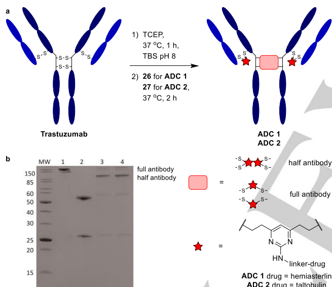
Scheme 5 a) Synthesis of ADC 1 and ADC 2 . b) SDS-PAGE analysis of the two ADCs; lane 1 is non-reducing, lanes 2-4 are reducing; lanes: MW = molecular weight marker, (1) trastuzumab, (2) reduced trastuzumab, (3) ADC 1 , (4) ADC 2 . TCEP = tris(2-carboxyethyl)phosphine. TBS = Tris-buffered saline (TrisHCl 25 mM, NaCl, 25 mM, EDTA 0.5 mM pH 8).
