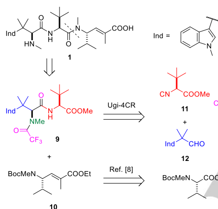
Scheme 1 Retrosynthetic analysis of hemiasterlin ( 1 )
