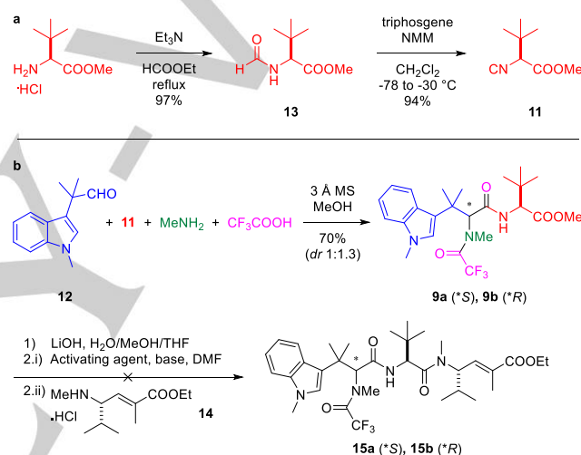
Scheme 2 a) Synthesis of isonitrile 11 b) The four-component Ugi reaction and the subsequent failed fragment amide coupling. NMM = N -methylmorpholine, MS = molecular sieves, THF = tetrahydrofuran, DMF = N,N -dimethylformamide
