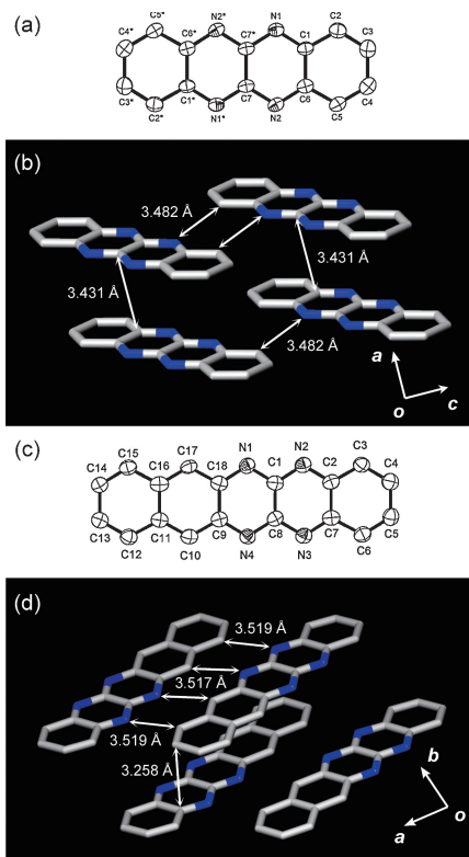
Figure 1. ORTEP drawings and single crystal structures of TANC (a) and (b) and BTANC (c) and (d).
