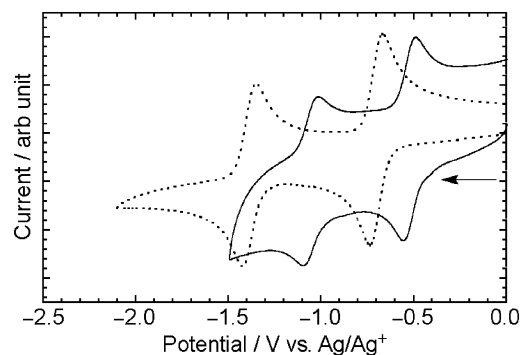
Figure 2. Cyclic voltammograms of TANC (dotted line) and BTANC (solid line) at 1.0 mM in \text{CH}_3\text{CN} solutions of n\text{-Bu}_4\text{NPF}_6 (0.10 M). Sweep rate is 100 \text{ mV s}^{-1} .
