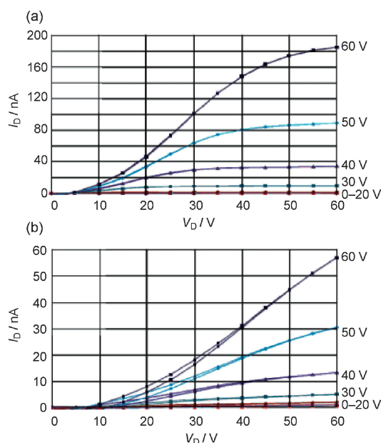
Figure 3. FET characteristics for the thin-films of (a) BTANC and (b) TANC. Gate voltages V_G were applied from 0 to 60 V in increments of 10 V.
