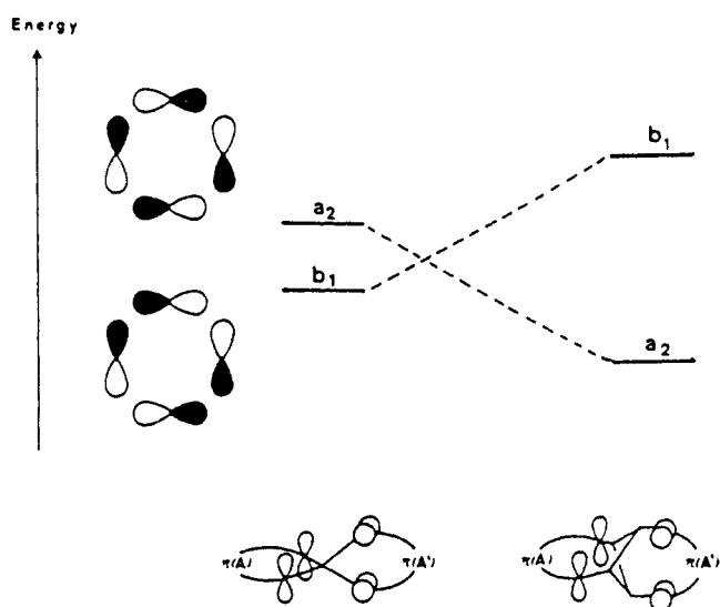
Figure 1. Orbital sequence for b 1 and a 2 in spiro compounds (left) and the corresponding tricyclic compounds (right).
