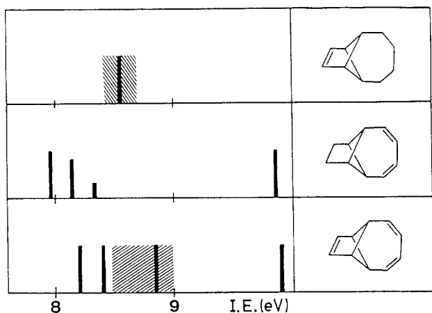
Figure 7. Comparison between the first bands in the PE spectra of 13 , 15 , and 16 .
