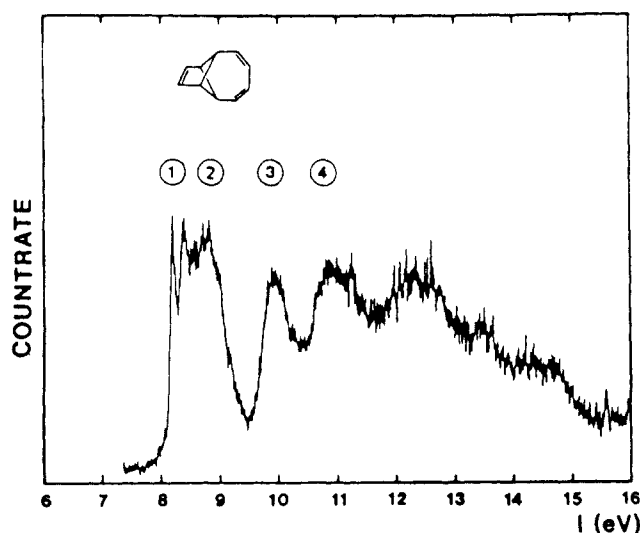
Figure 6. He ( I_a ) PE spectrum of 13.
