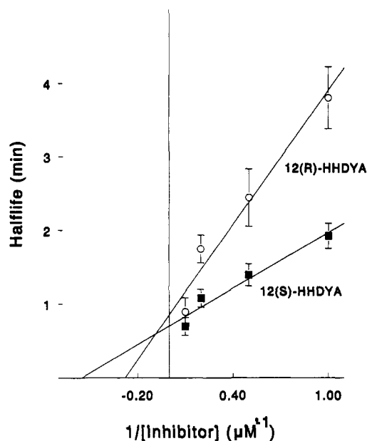
Figure 2. Determination of the K_I and t_{1/2} values for the inactivation of prostaglandin \omega -hydroxylase (CYP4A4) by the 12S and 12R enantiomers of 12-hydroxy-16-heptadecynoic acid. The Y-axis values for the points on the plot were obtained by weighed linear regression analysis of the time points between 0 and 1.5 min in Figure 1.
