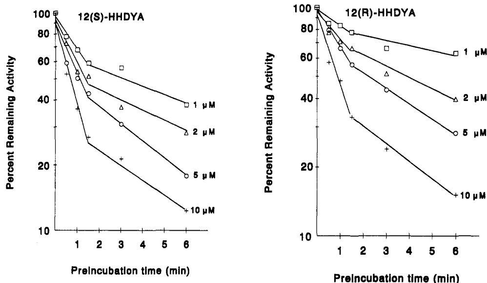
Figure 1. Time-dependence of the inactivation of prostaglandin E_1 \omega -hydroxylase (CYP4A4) by (S)- and (R)-12-hydroxy-16-heptadecynoic acid. The concentrations of the inhibitors in the preincubation mixtures are indicated in the figures.
