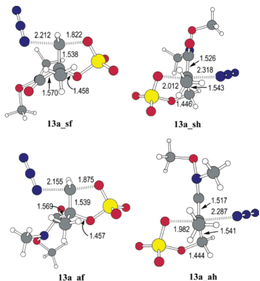
FIGURE 2. Some geometrical features of the TS 13a , calculated at the B3LYP/6-31+G(d) level.
