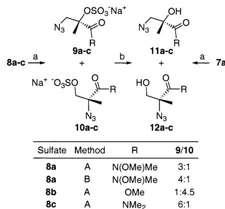
SCHEME 3. Ring-Opening Reactions of Cyclic Sulfates 8a–c with the Azide Ion a
