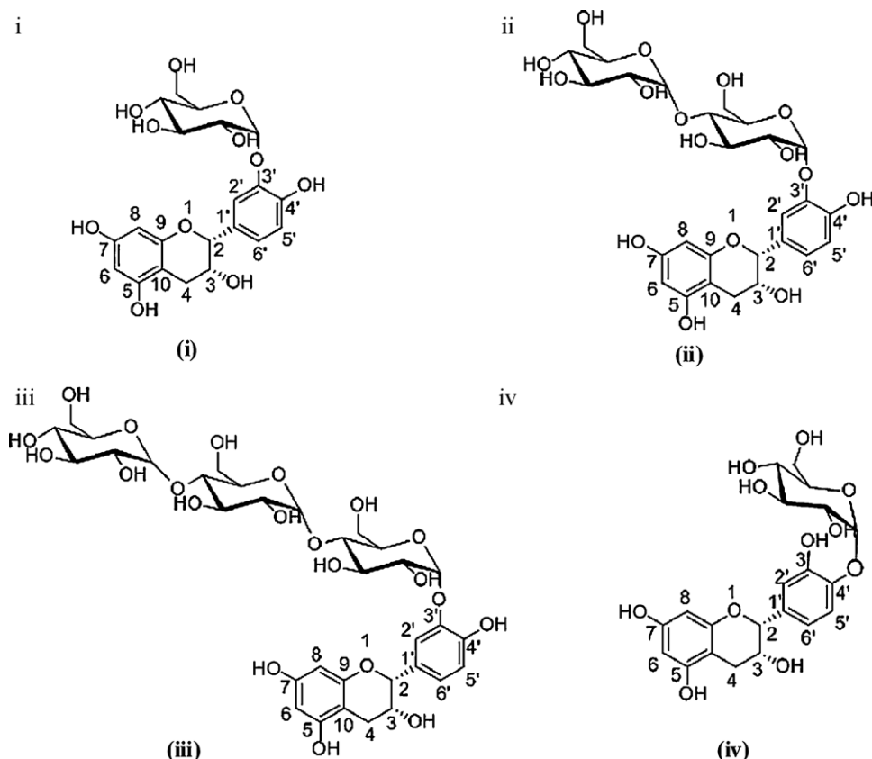
Fig. 7. Proposed structure of the products (i) (–)-EC-3'-O-α-D-glucopyranoside (EC3A), (ii) (–)-EC-3'-O-α-D-digluco-pyranoside (EC3B), (iii) (–)-EC-3'-O-α-D-trigluco-pyranoside (EC3C) and (iv) (–)-EC-4'-O-α-D-glucopyranoside (EC4A).
