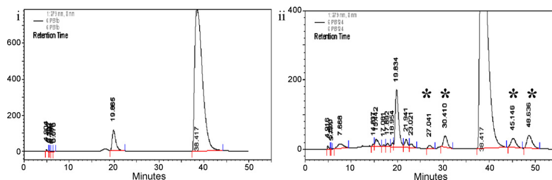
Fig. 3. HPLC chromatogram of the reaction products of EC and \beta -CD catalyzed by the CGTase from Paenibacillus sp. RB01 after (i) 0 and (ii) 24 h incubation. The asterisk (*) marks the EC-glucosides.
