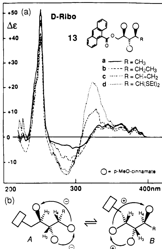
Figure 4. (a) CD spectra of four 1,2,3,4-tetrol derivatives with D-ribo stereochemistry and different alkyl substituents (R). (b) Major "sickle" conformations and their corresponding exciton chiralities in D-ribo derivatives as determined by NMR analysis.
