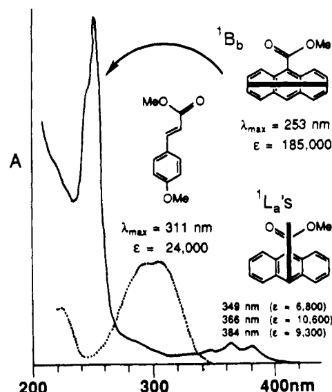
Figure 1. UV absorption spectra and associated transitions of 9-anthroate and p -methoxycinnamate chromophores (not shown to scale).
