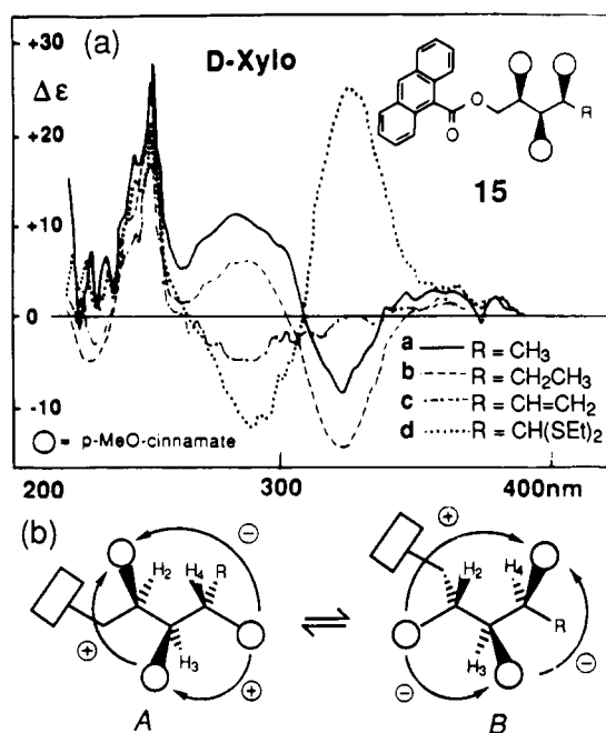
Figure 6. (a) CD spectra of four tetrol derivatives with D-xylo stereochemistry with varying alkyl substituents. Note that the variable spectral pattern in this series requires that any tetrol derivative with unknown configuration be compared to those derivatives with the most similar alkyl group, i.e., the curve of an unknown having a C-5 methylene should be compared to the curves of 13b–16b . (b) Major "sickle" conformations and their corresponding exciton chiralities in D-xylo derivatives as determined by NMR analysis. Conformation A, with a net positive exciton chirality, dominates in 15d , while conformation B, with a net negative exciton chirality, dominates in 15a,b .
