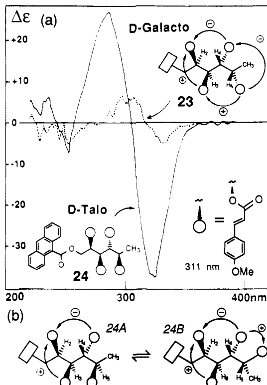
Figure 11. (a) CD spectra of 1,2,3,4,5-pentol derivatives with D-galacto and D-talo stereochemistry. (b) Major conformations of D-talo derivative 24 , as determined by NMR: extended ("zigzag") conformation 24A and bent ("sickle") conformation 24B .
