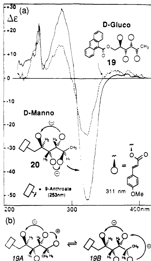
Figure 9. (a) CD spectra of 1,2,3,4,5-pentol derivatives with D-glucoside and D-mannoside stereochemistry. (b) Major conformations of D-glucoside 19, as determined by NMR: bent ("sickle") conformation 19A and extended ("zigzag") conformation 19B. The net negative C/C coupling in both derivatives is indicated by the signs of the pairwise interactions.
