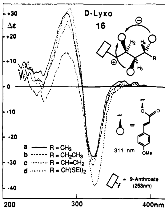
Figure 7. CD spectra of tetrol derivatives with D-lyxo stereochemistry.
