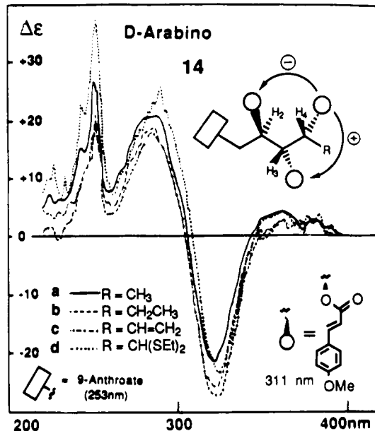
Figure 5. CD spectra of tetrol derivatives with D-arabino stereochemistry.
