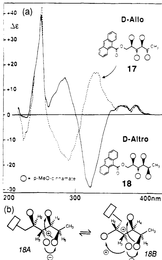
Figure 8. (a) CD spectra of 1,2,3,4,5-pentol derivatives with D-allo and D-altro stereochemistry. (b) Major conformations and their corresponding pairwise exciton chiralities of D-altro derivative 18, as determined by NMR: extended ("zigzag") conformation 18A and bent ("sickle") conformation 18B.
