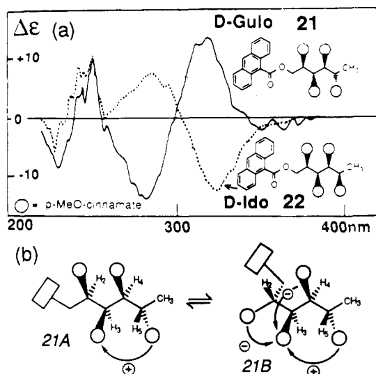
Figure 10. (a) CD spectra of 1,2,3,4,5-pentol derivatives with D-gulo and D-ido stereochemistry. (b) Major conformations of D-gulo derivative 21 , as determined by NMR: extended ("zigzag") conformation 21A and bent ("sickle") conformation 21B .
