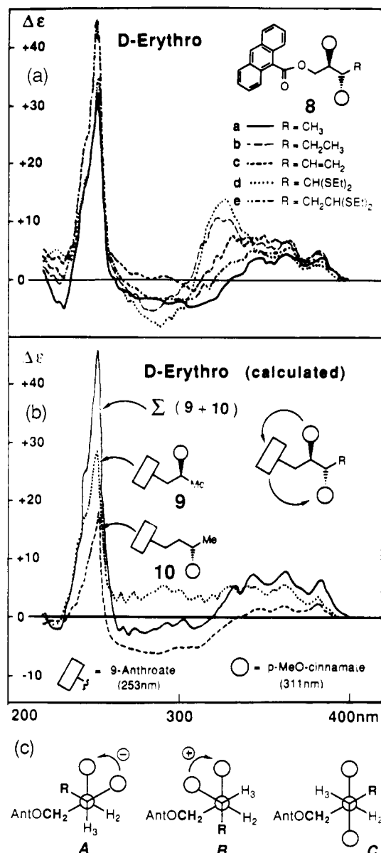
Figure 2. Circular dichroic spectra of "bichromophorically derivatized" D-erythro 1,2,3-triols 8 : (a) Reference curves for empirical assignment of relative and absolute configuration. (b) Simulated curve from summation of 1,2- and 1,3-anthracene/cinnamate pairwise interactions represented by 9 and 10 , respectively. (c) Three C-2/C-3 rotamers dictating minimal net cinnamate/cinnamate exciton coupling.
