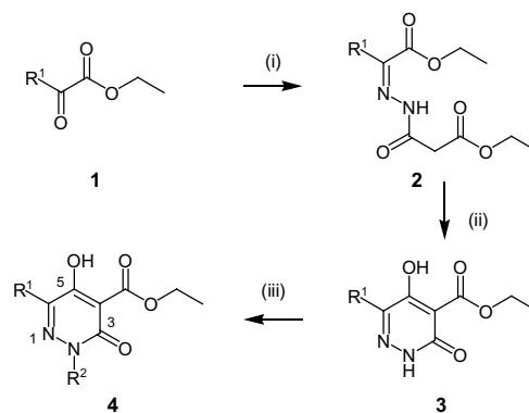
Scheme 1. Reagents and conditions: (i) Hydrazinocarbonyl-acetic acid ethyl ester, DMSO, 0.4% TFA (v/v), 70 °C, 16 h; (ii) NaOAc, DMF, 150 °C, 30 min, –2 h; (iii) NaH, DMF, 25 °C, 10 min followed by addition of electrophiles, then heating (if needed).
