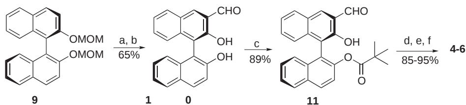
Scheme 1. (a) t\text{-BuLi} , DMF, THF, -78^\circ\text{C} ; (b) \text{HCl} , EtOH; (c) \text{NaH} , pivaloyl chloride, THF; (d) diamine, EtOH, reflux; (e) \text{Mn}(\text{OAc})_2 , EtOH, reflux, \text{O}_2 ; (f) \text{LiCl} , EtOH.
