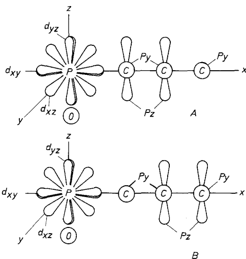
Abb. 1. A 1- DEPP -Carbanion; B Allen-Carbanion
