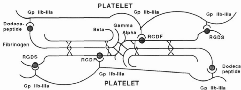
Figure 1. Platelet-platelet interaction mediated by fibrinogen.
