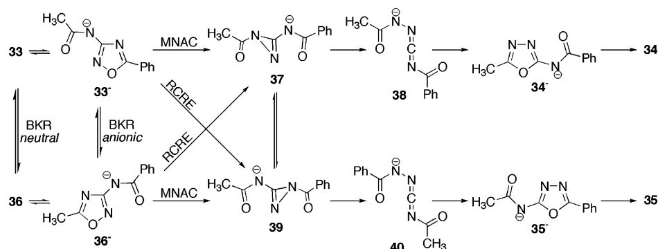
SCHEME 8. Competition between BKR, MNAC, and RCRE Routes in the Rearrangements of Oxadiazoles 33 and 36
