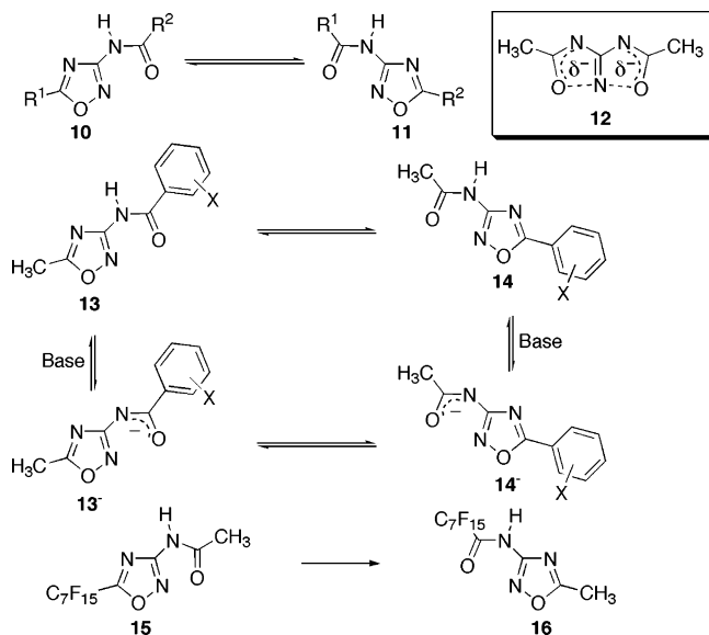
SCHEME 3. General Scheme and Examples of Ring-Degenerate BKR of 1,2,4-Oxadiazoles
