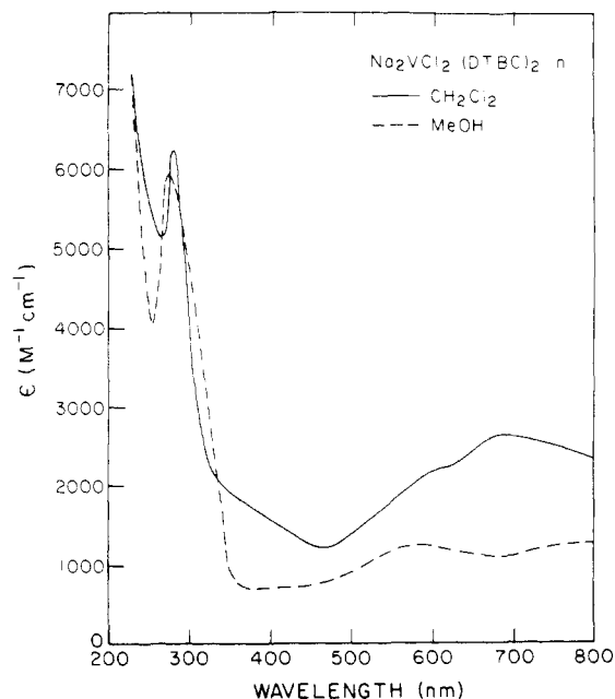
Figure 6. Absorption spectra of 1 mM solutions of \text{Na}_2\text{V}^{\text{IV}}\text{Cl}_2(\text{DTBC})_2 in (a) \text{CH}_2\text{Cl}_2 and (b) \text{MeOH} .
