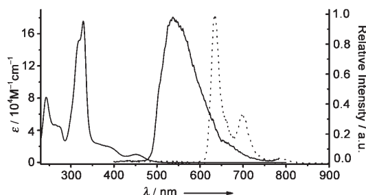
Figure 7. UV/Vis absorption (—), normalized fluorescence (—) and phosphorescence (.....) spectra of KGd(Az) 4 in CH 3 CN (UV/Vis: room temperature; fluorescence: M = 1.2 \times 10^{-5} mol L −1 , \lambda_{\text{ex}} = 400 nm, 298 K; phosphorescence: \lambda_{\text{ex}} = 400 nm, 77 K, delay time 0.01 ms, gate time 20 ms).
