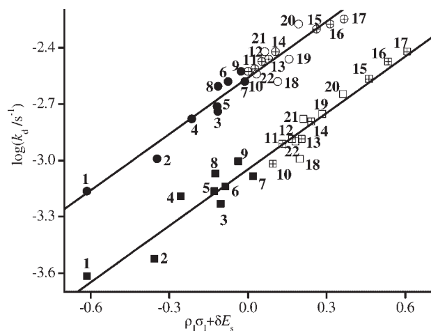
Figure 2. Plot of \log(k_d/s^{-1}) at 120 °C versus Eqns 23(a) (square) and 23(b) (circle), (■, □, ⊞) RR/SS isomers, (●, ○, ⊕) RS/SR isomers, for alkoxyamines 1–9 (filled symbols), 10–17 (crossed symbols), and 18–22 (open symbols)
