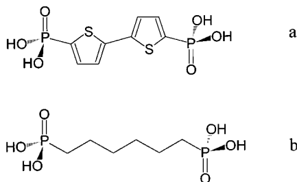
Scheme 1. Structures of Bis(phosphonates): (a) 2,2'-Bithiophene-5,5'-diylbis(phosphonic acid) (BDP) and (b) 1,6-Hexanediylbis(phosphonic acid) (HBPA)
