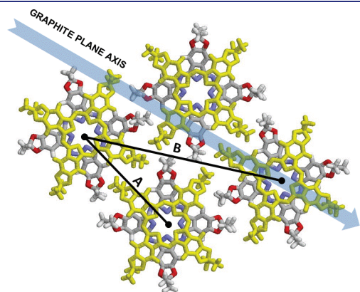
Figure 4. Scheme of the 2D aggregation of \text{Pc}_2\text{Tb} complexes on HOPG obtained from MD simulations (the terbium ions are not shown). The \text{Pc}^{2-} lying directly on graphite (depicted in yellow) has one arm on average parallel to the graphite axis, and this direction corresponds to the favorite direction of growth of the aggregate. The uppermost \text{Pc}^{2-} (colored following the Corey–Pauling–Koltun scheme) is twisted by about 45^\circ with respect to the growth direction. These 2D crystals present an approximately hexagonal lattice with side A = 19.5 \pm 1 \text{ \AA} ( B = 33 \pm 2 \text{ \AA} ).
