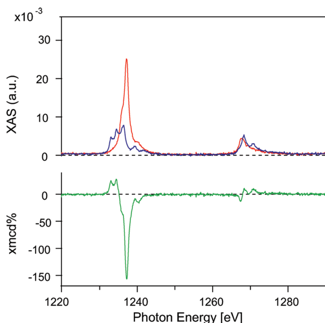
Figure 9. XAS spectra at the M_{4,5} edge of Tb for ML1 with helicities parallel ( I_{\parallel}^{\parallel} , in red) and antiparallel ( I_{\parallel}^{\perp} , in blue) to an applied magnetic field of 5 T at 7 K (above), and the XMCD spectrum given by their difference normalized to the maximum intensity of the unpolarized spectrum 1/2(I_{\parallel}^{\parallel} + I_{\parallel}^{\perp}) (below in green). 42
