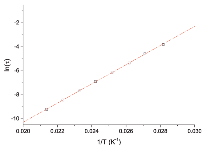
Figure 7. Arrhenius plot of the natural logarithm of the relaxation time \tau of complex 1 .
