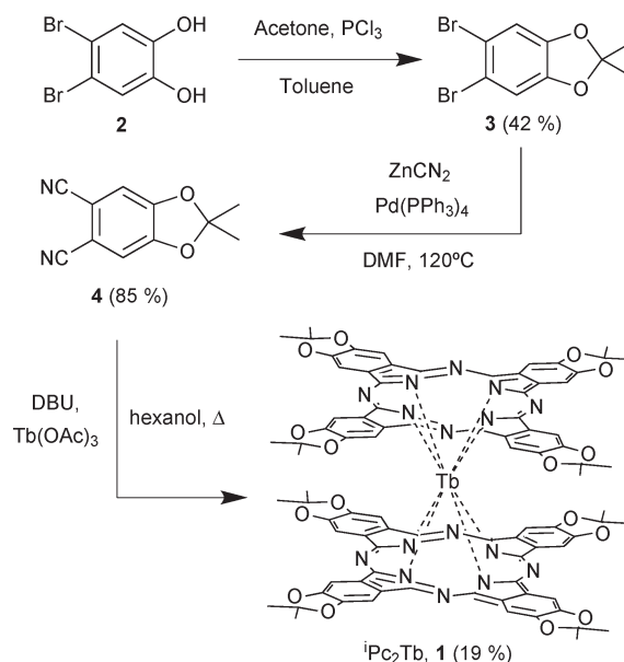
Scheme 1. Synthesis of {}^i\text{Pc}_2\text{Tb} (1) in Three Steps From 4,5-Dibromocatechol (2) Using a One-Step Methodology from the Corresponding Phthalonitrile 4
