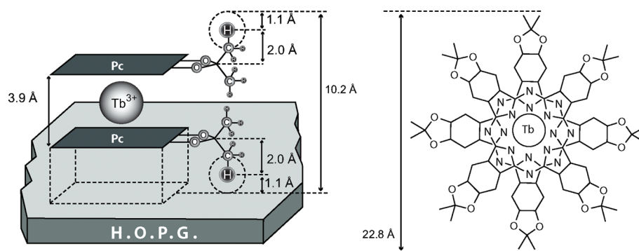
Figure 2. Schematic representation of complex {}^i\text{Pc}_2\text{Tb} on top of the graphite (left) and the lateral dimensions of the complex (right).
