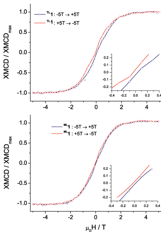
Figure 10. XMCD detected hysteresis of magnetization for the thick layer sample TL1 (above) and the monolayer sample ML1 (below) on HOPG measured at 7 K (see text). The inset shows the enlargement of the central part of both hystereses.
