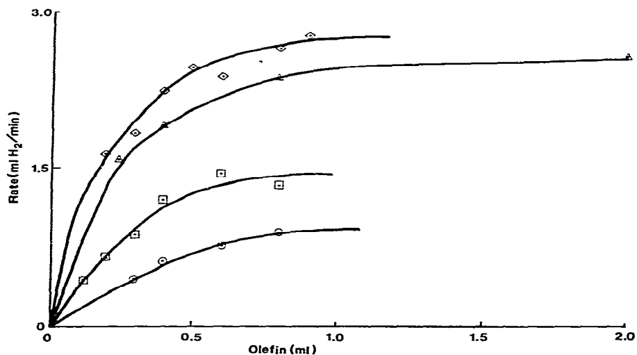
Fig. 4. The rate of hydrogenation of 1-hexene as a function of [Ru] and [olefin]. Data refer to sample R2 ( \circ 100 mg, \square 150 mg, \triangle 300 mg) or \text{RuCl}_2(\text{PPh}_3)_3 ( \diamond 23.3 mg).
