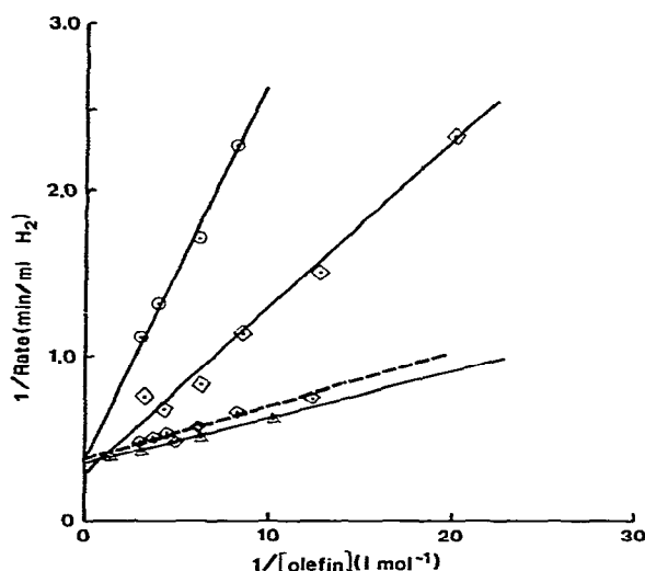
Fig. 5. Plot of 1/[\text{olefin}] vs. 1/\text{rate} for the hydrogenation of 1-hexene. Data refer to sample R2 ( \circ 100 mg, \square 150 mg, \triangle 300 mg) or \text{RuCl}_2(\text{PPh}_3)_3 ( \diamond 23.3 mg).
