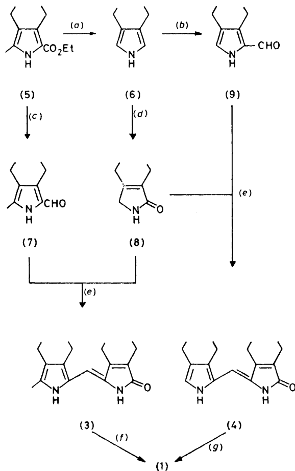
SCHEME 2 Syntheses of octaethylbilindione. (a) (i) \text{SO}_2\text{Cl}_2 ; (ii) aqueous NaOH; (iii) heat, catalyst (yield 74.5%, ref. 13; we observed similar yields); (b) \text{POCl}_3 -DMF; (c) (i) aqueous NaOH; (ii) \text{POCl}_3 -DMF (yield 44%, ref. 14; we observed similar yields); (d) \text{H}_2\text{O}_2 -pyridine; (e) NaOH-EtOH (f) \text{O}_2 -HOAc; (g) \text{HC}(\text{OMe})_3 -HCl
