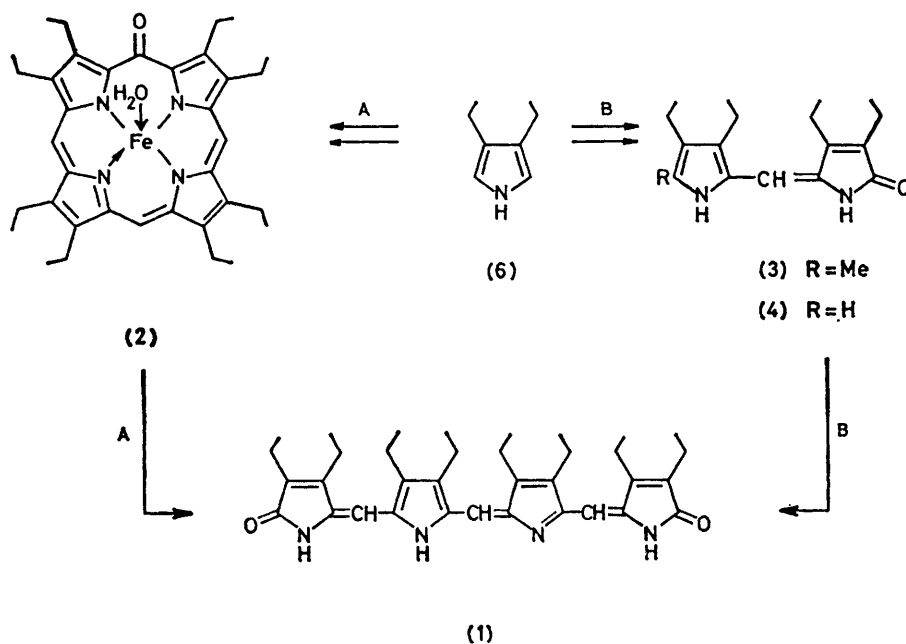
SCHEME 1 Alternative approaches to octaethylbilindione; A = biomimetic route; B = pyrromethenone route
