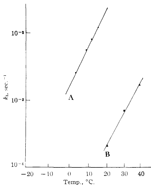
Fig. 2.—Arrhenius plots for the neutral hydrolysis of dimethylcarbamyl chloride (A) and ethyl chloroformate (B).
