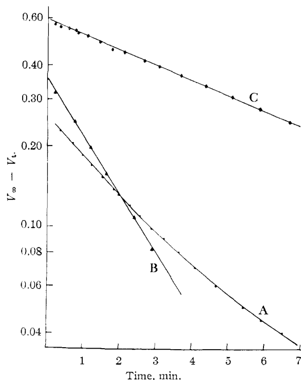
Fig. 1.—Representative first-order hydrolysis rate plots: A, dimethylcarbamyl chloride (Table I, expt. 4); B, dimethylcarbamyl chloride in presence of alkali (expt. 10); C, ethyl chloroformate (expt. 18) (multiply time scale by ten).
