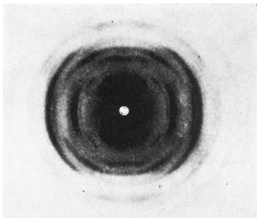
Fig. 1.—X-Ray diffraction photograph of a sodium pectate fiber: \text{CuK}\alpha radiation; fiber axis vertical; camera distance 5.0 cm.
