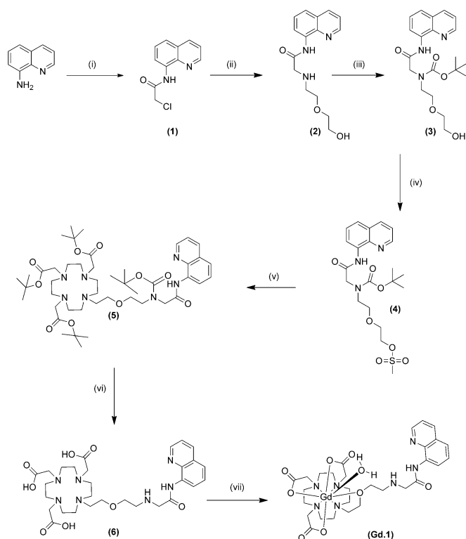
Scheme 1. Formation of Gd-1. i) Chloroacetyl chloride, pyridine/ \text{CHCl}_3 (79%). ii) 2-(2-Aminoethoxy)ethanol, DIPEA, KI, MeCN (90%). iii) Boc anhydride, pyridine, THF (90%). iv) Methane sulfonyl chloride, DCM, triethylamine (90%). v) t Bu DO 3 A, K 2 CO 3 , DCM, (77%). vi) TFA, DCM (> 99%). vii) GdCl 3 ·6H 2 O, H 2 O, pH 5.5 (91%).
