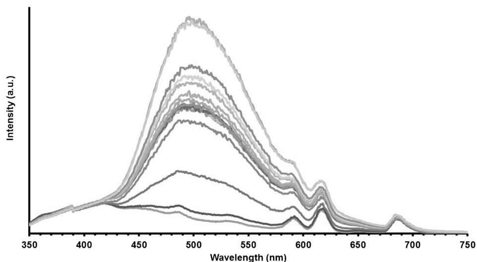
Figure 3. Eu-1 versus \text{Zn}^{\text{II}} fluorescence (1 mM, pH 7.4, 298 K, \lambda = 280 nm).
