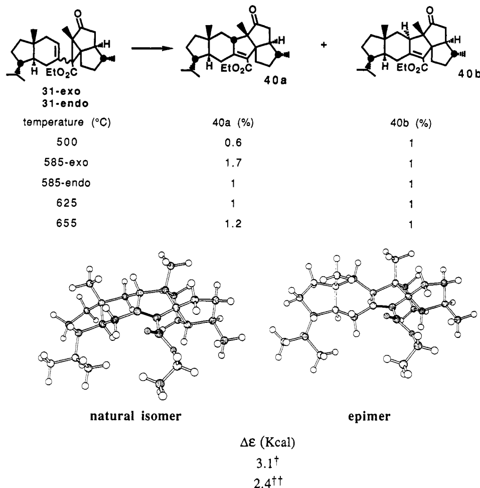
Figure 9. MM2 conformations for 40a and 40b and the temperature profile for the rearrangement.
