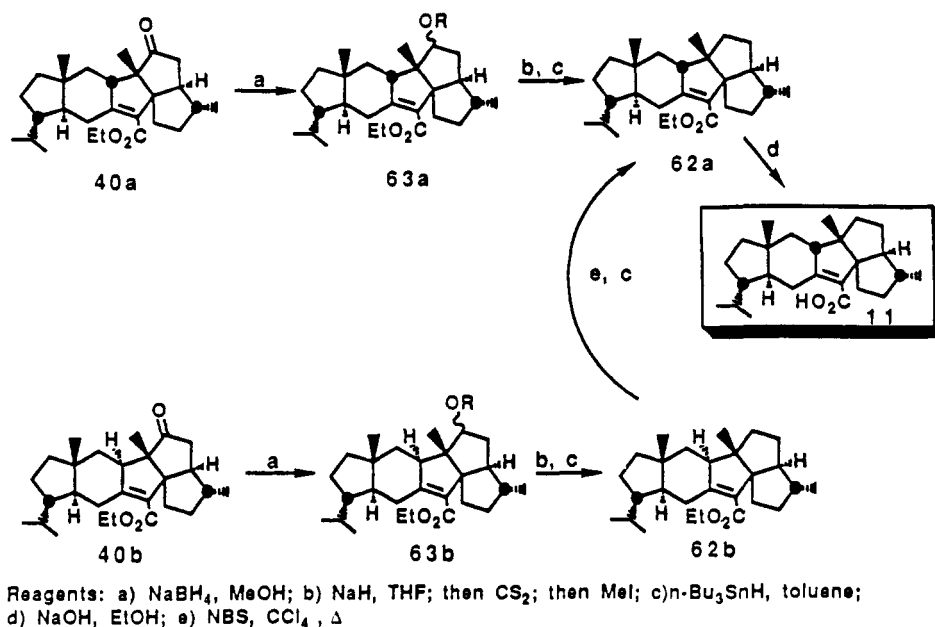
Figure 10. Synthesis of retigeranic acid.
