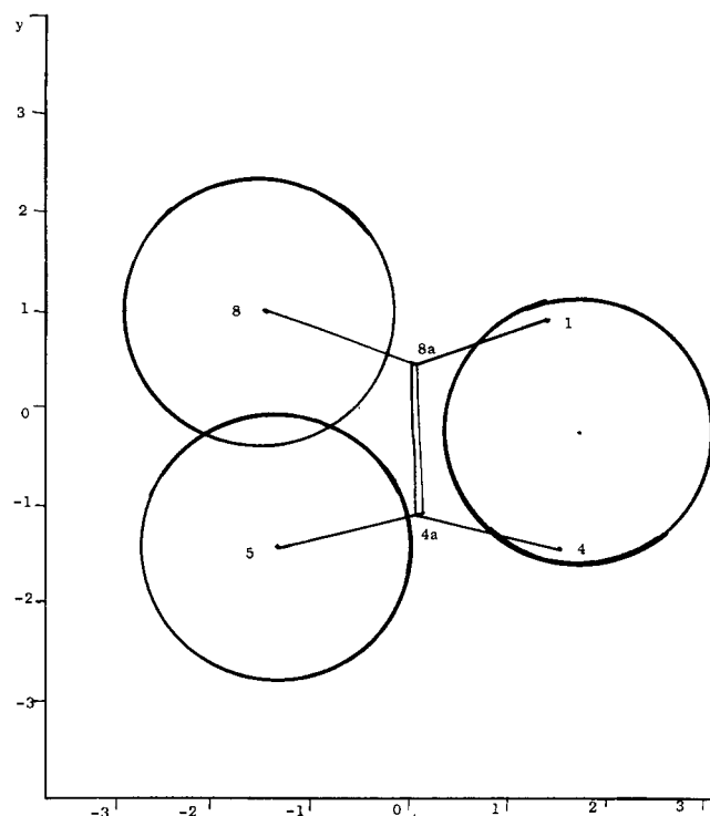
Figure 2. View from above toward the C=C bond of 1 . Circles represent 1.2-Å van der Waals radius of blocking hydrogen atoms H(6), H(7), and H(10).
