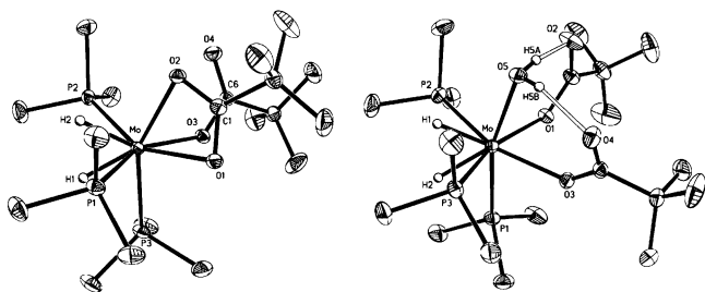
Figure 1. Molecular structures of \text{Mo}(\text{PMe}_3)_3(\eta^2\text{-O}_2\text{CBu}^t)(\eta^1\text{-O}_2\text{CBu}^t)\text{H}_2 and \text{Mo}(\text{PMe}_3)_3(\eta^1\text{-O}_2\text{CBu}^t)_2(\text{OH}_2)\text{H}_2 .
