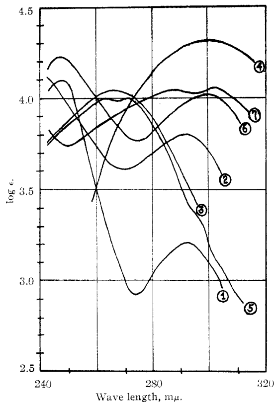
Fig. 1.—Ultraviolet absorption spectra of: (1) \beta -(1-tetralone-2)-butyric acid (II); (2) \beta -(1-amino-3,4-dihydro-2-naphthalene)-butyrolactam (III); (3) \beta -(1-carbomethoxymethyl-3,4-dihydro-2-naphthyl)-butyric acid (VI); (4) 1-methyl-3-keto-1,2,3,9,10,10a-hexahydrophenanthrene (XI); (5) 1-methyl-3-keto-4-carbomethoxy-1,2,3,4,9,10-hexahydrophenanthrene (X); (6) enolate of X; (7) 1-methyl-2-carbomethoxy-3-keto-1,2,3,9,10,10a-hexahydrophenanthrene.
