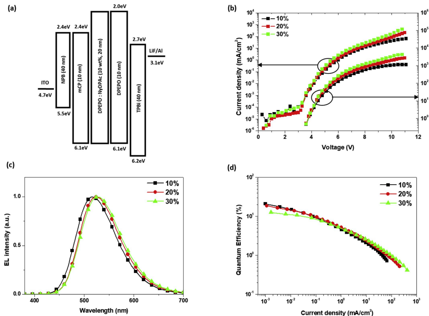
Fig. 3. (a) Energy level diagram for the OLED device, (b) current density-voltage-luminance (J-V-L) curves, (c) EL spectra at 5 V, (d) external quantum efficiency-current density ( \eta_{\text{EQE}}-J ) curve.
