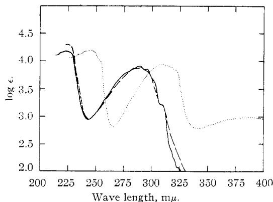
Fig. 2.—Spectra of: . . . . . 7-methyl-7H-pyrrolo[2,3-b]pyridine; —, 1-methyl-7-azaindole; ----, 7-azaskatole.
