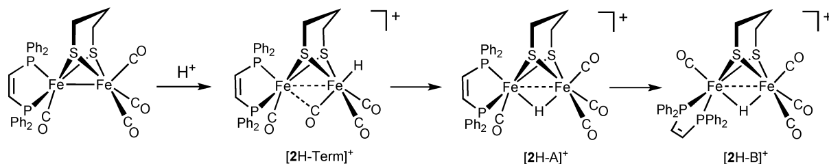
Scheme 2 Course of protonation of 2 , \text{Fe}_2(\text{pdt})(\text{CO})_4(\text{dppv}) .
