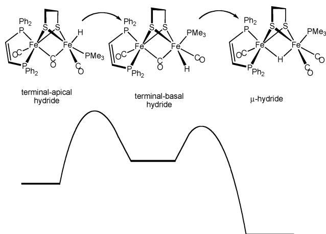
Scheme 8 Schematic reaction coordinate for the isomerization of the apical-terminal hydrides. Basal-terminal hydrides are not observed, indicating their rapid conversion to the μ-hydrides.
