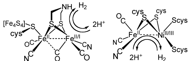
Fig. 1 Structures and reactivity of the [\text{FeFe}] - and [\text{NiFe}] -hydrogenases with proposed oxidation states.
