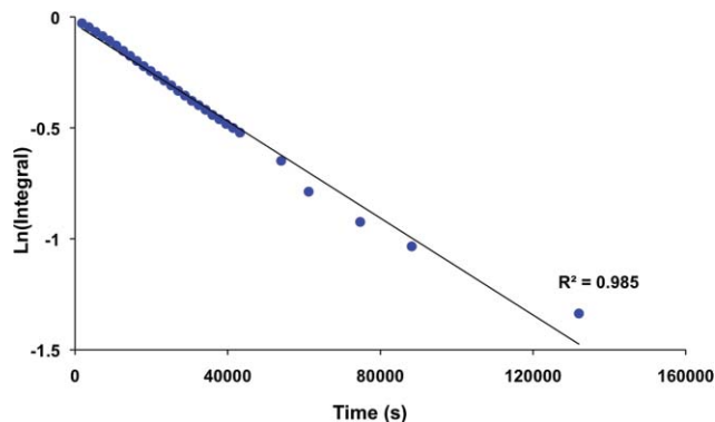
Fig. 4 Plot of the isomerization of [\text{4H-B}]^+ to [\text{4H-C}]^+ , as monitored by ^1\text{H} NMR spectroscopy.
