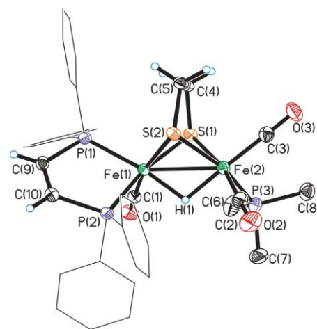
Fig. 2 Structure of the cation in [Fe_2(edt)(\mu-H)(CO)_3(dppv)(PMe_3)]PF_6 ( [3H-B]^+ ) with thermal ellipsoids drawn at the 50% probability level, phenyl hydrogen atoms omitted for clarity. Key distances (Å): Fe–Fe, 2.5744 (5); Fe(1)–S(1), 2.2581 (7); Fe(1)–S(2), 2.2794 (6); Fe(2)–S(1), 2.2668 (7); Fe(2)–S(2), 2.2760 (6); Fe(1)–P(1), 2.2137 (6); Fe(1)–P(2), 2.2282 (6); Fe(1)–H(1), 1.69 (2); Fe(2)–H(1), 1.64 (2).
