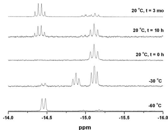
Fig. 3 ^1\text{H} -NMR spectra ( \text{CD}_2\text{Cl}_2 , 500 MHz) for protonation of \text{Fe}_2(\text{pdt})(\text{CO})_3(\text{dppv})(\text{PMe}_3) ( 4 ) with \text{HBF}_4 \cdot \text{Et}_2\text{O} and various stages in the isomerization of the resulting hydrides.
