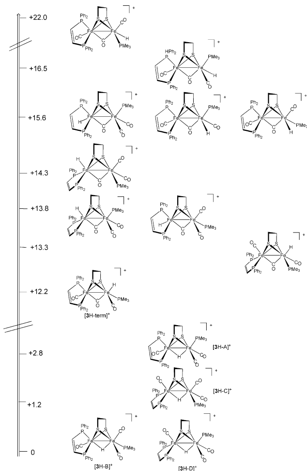
Scheme 5 Computed relative thermodynamic stability of relevant [(\text{dppv})(\text{CO})\text{Fe}(\text{edt})\text{Fe}(\text{CO})_2(\text{PMe}_3)(\text{H})]^+ isomers, energies in kcal/mol.
