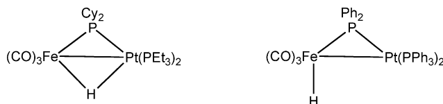
Scheme 1 Two isomers of \text{HFe}(\text{CO})_3(\mu\text{-PR}_2)\text{Pt}(\text{PR}'_3)_2 .
