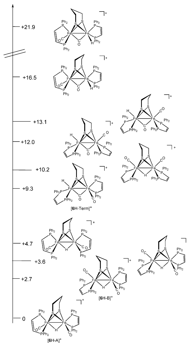
Scheme 7 Computed relative thermodynamic stability of relevant [(\text{dppv})(\text{CO})\text{Fe}(\text{edt})\text{Fe}(\text{CO})(\text{dppv})(\text{H})]^+ isomers, energies in kcal/mol.
