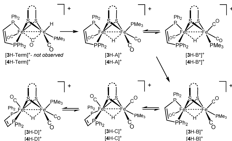
Scheme 3 Isomerization pathway for [HFe_2(pdt)(CO)_3(dppv)(PMe_3)]^+ , [4H]^+ , and [HFe_2(edt)(CO)_3(dppv)(PMe_3)]^+ , [3H]^+ , and their equilibrium isomer distribution.
