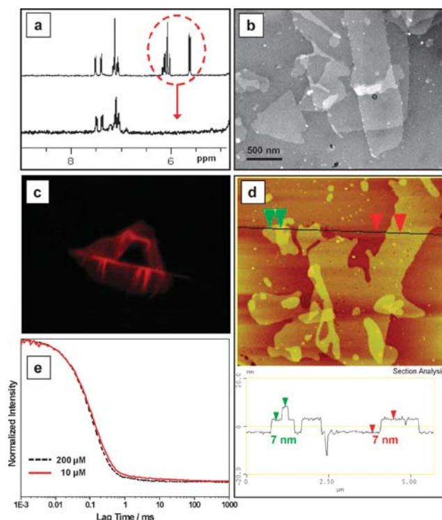
Fig. 2 (a) 1 H-NMR spectra of 1 (upper) and polymerized 1 (lower) in D 2 O. The 1 H-NMR spectrum of polymerized 1 reveals complete disappearance of the acrylic double bond at around 6 ppm. (b) TEM image of polymerized objects of 1 with negative staining. (c) Fluorescence microscopy image of polymerized sheets of 1 encapsulating Nile Red in aqueous solution. (d) AFM image of polymerized sheets of 1 with height information. (e) Autocorrelation functions of an aqueous solution of polymerized objects of 1 with different concentrations.
