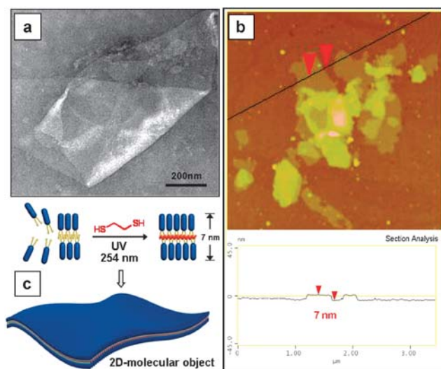
Fig. 1 (a) TEM image of self-assembled sheets of 1 . (b) AFM image of self-assembled sheets of 1 with height information. (c) Schematic representation of the confined polymerization of 2D peptide sheets.
