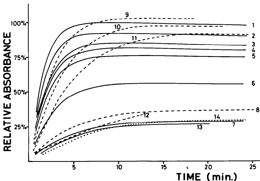
Fig. 2. Relative E_{624} vs time of 1.86 \times 10^{-5} M solns of 7 ( A^- = CF_3COO^- )/air at 25^\circ in: (1) H_2O -satd CHCl_3 ; (2) CaCl_2/K_2CO_3 -dried CHCl_3 ; (2–6) in mixtures of H_2O -satd CHCl_3 and CaCl_2/K_2CO_3 -dried CHCl_3 in the ratios of 5:1 (2); 2:1 (3); 1:1 (4); 1:2 (5); 1:5 (6); (8) in CaCl_2/K_2CO_3 -dried CHCl_3/MeCN (0.7% instead of 0.4%); (9–12) in H_2O -satd CHCl_3/EtOH (0.1% (9), 0.2% (10); 0.3% (11); 1.0% (12)). (The final dilutions 1–7 and 9–12 contained 0.4% of reagent grade MeCN ( H_2O < 0.05\% ). Starting from a stock soln of the salt in freshly distilled MeCN and diluting with dried CHCl_3 gave curves 13 and 14, which have to be compared with curves 7 and 8, respectively).
