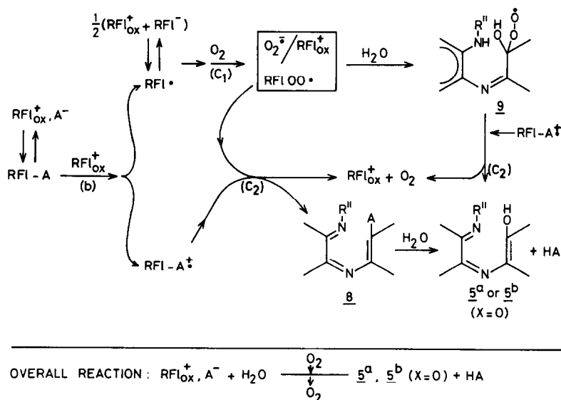
Scheme 4. The 10,10' -ring opening is coupled with or followed by the transfer of an electron from a peroxy radical to the radical cation RFI-A^+ .
