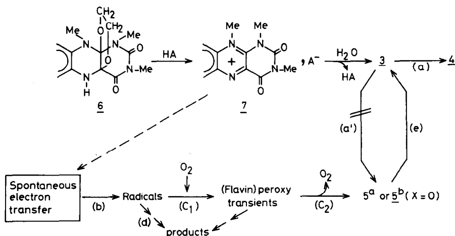
Scheme 2. Blue-colouration (formation of 5^a or 5^b ) indicating the occurrence of electron transfer and O_2 -activation in 1,3,10-trimethylalloxazinium salt solutions.
