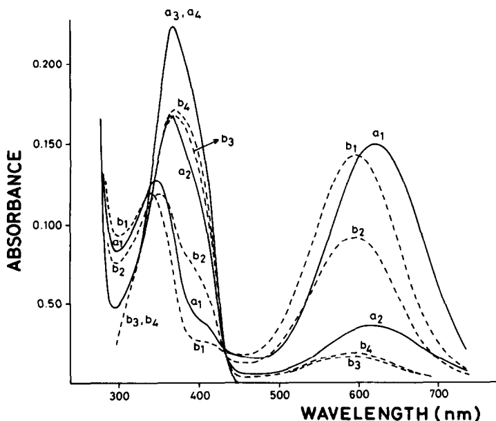
Fig. 1. Spectra recorded at maximal blue colouration of 1.86 \times 10^{-5} M solns of 7 ( A^- = CF_3COO^- ) at 25° in: (a 1 ) H_2O -satd CHCl_3 /air; (a 2 ) CaCl_2/K_2CO_3 -dried CHCl_3 /air; (a 3 ) H_2O -satd CHCl_3/N_2 ; (a 4 ) CaCl_2/K_2CO_3 -dried CHCl_3/N_2 ; (b 1 ) H_2O -satd benzene/air; (b 2 ) sodium-dried benzene/air; (b 3 ) H_2O -satd benzene/ N_2 ; (b 4 ) sodium-dried benzene/ N_2 . (Procedure: MeCN-stock solns of the salt were diluted with CHCl_3 or benzene in the ratio of 1:250).
