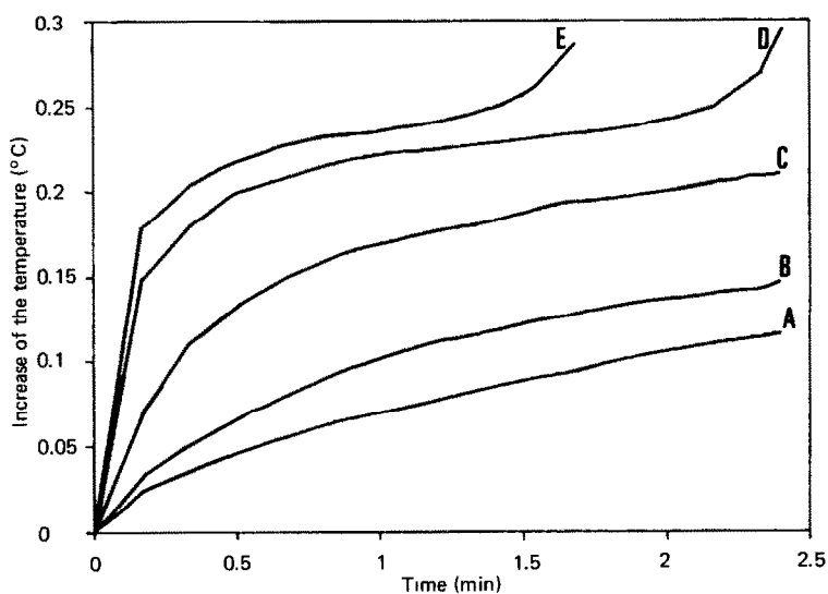
Fig. 8. Thermometric curves of the \text{V}^{\text{V}} catalysed reaction ( [\text{BrO}_3^-] = 0.07 \text{ M} ; [\text{I}^-] = 0.01 \text{ M} ; [ascorbic acid] = 0.01 \text{ M} ; [\text{H}_2\text{SO}_4] = 0.01 \text{ M} ): curve A, [\text{V(V)}] = 2.8 \text{ ppm} ; curve B, [\text{V(V)}] = 5.5 \text{ ppm} ; curve C, [\text{V(V)}] = 14 \text{ ppm} ; curve D, [\text{V(V)}] = 56 \text{ ppm} ; curve E, [\text{V(V)}] = 70 \text{ ppm} .
