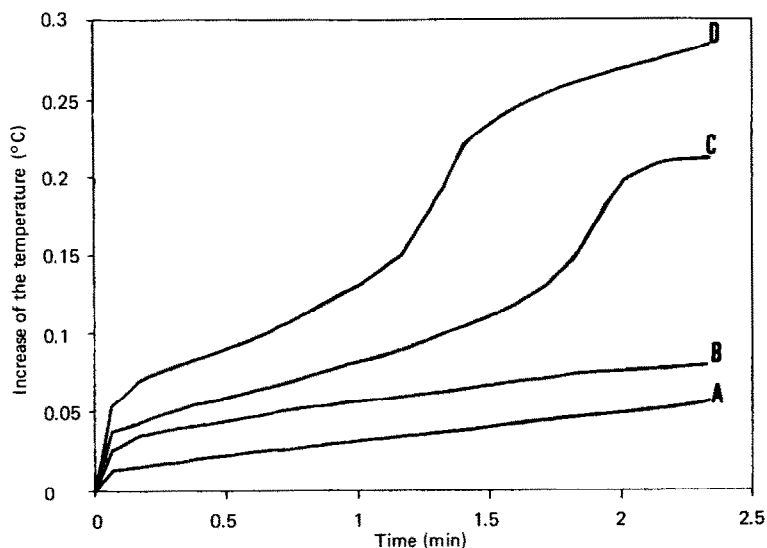
Fig. 7. Thermometric curves of the \text{Ru}^{\text{III}} catalysed reaction ( [\text{BrO}_3^-] = 0.07 \text{ M} ; [\text{I}^-] = 0.01 \text{ M} ; [ascorbic acid] = 0.01 \text{ M} ; [\text{H}_2\text{SO}_4] = 0.01 \text{ M} ): curve A, [\text{Ru(III)}] = 3.9 \text{ ppm} ; curve B, [\text{Ru(III)}] = 7.8 \text{ ppm} ; curve C, [\text{Ru(III)}] = 9.76 \text{ ppm} ; curve D, [\text{Ru(III)}] = 13.7 \text{ ppm} .
