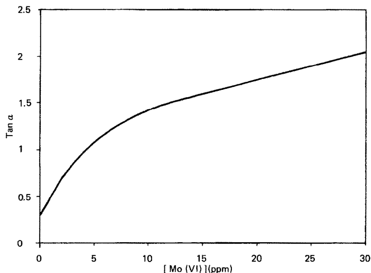
Fig. 6. Study of the linearity of the response ( [\text{BrO}_3^-] = 0.07 \text{ M} ; [ascorbic acid] = 0.01 \text{ M} ; [\text{I}^-] = 0.01 \text{ M} ; [\text{H}_2\text{SO}_4] = 0.01 \text{ M} ).
