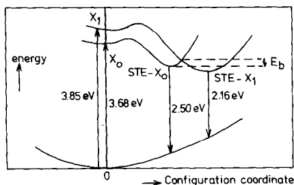
Fig. 5. Configuration coordinate diagram of \Gamma excitons in \text{CdI}_2 . X_0 and X_1 are free excitons of symmetry \Gamma_{6a}^- and \Gamma_{8a}^-/\Gamma_{8s}^- , observed in reflection (20). The corresponding self-trapped excitons \text{STE}-X_0 and \text{STE}-X_1 are responsible for luminescence at 2.50 and 2.16 eV, respectively.
