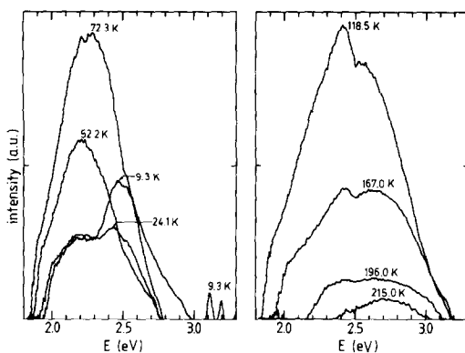
FIG. 1. Photoluminescence spectra of CdI 2 . The intensity of emission (arbitrary units) from single crystals is given as a function of photon energy. The emission output was corrected for instrumental effects. The excitation energy was 3.54 eV, with a spectral width of 0.02 eV.
