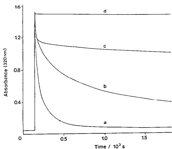
Fig. 1. Absorbance–time profiles recorded for a series of injections of a dilute \text{Ce}^{IV} solution ( 70 \text{ mm}^3 , 0.01 \text{ mol dm}^{-3} ) into 2.5 \text{ cm}^3 of a stirred dispersion of \text{RuO}_2 \cdot y\text{H}_2\text{O}^* ( 70 \text{ mg dm}^{-3} ) in 0.5 \text{ mol dm}^{-3} \text{ H}_2\text{SO}_4 , containing different concentrations of \text{Ce}^{III} ions: (a) 2.65 \times 10^{-4} , (b) 2.65 \times 10^{-3} , and (c) 2.65 \times 10^{-2} \text{ mol dm}^{-3} . The absorbance–time curve (d) was recorded using the same conditions as in (c), but in the absence of the redox catalyst.
