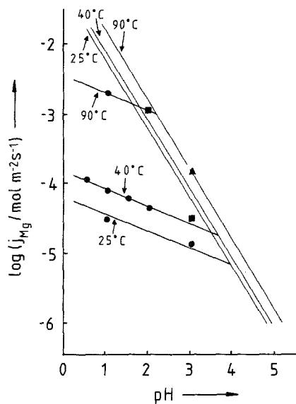
Fig. 2. Plots of \log (dissolution rate) vs. pH for MgO \{100\} . Thin lines: 1/2 j_{H^+} ( f = 10 \text{ s}^{-1} ). Chemical control \bullet ; chemical component of mixed kinetics \blacksquare ; diffusional control ( f = 10 \text{ s}^{-1} ) \blacktriangle
