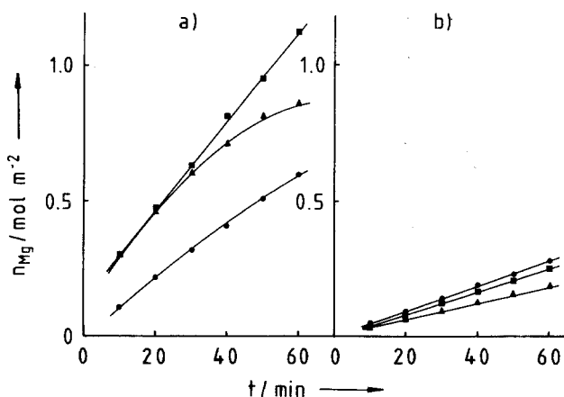
Fig. 1. Plots of amounts of \text{Mg}^{2+} dissolved vs. time at 40^\circ\text{C} and \text{pH} = 1.0 . a) Mechanically polished; b) Chemically polished \text{MgO} single crystals: {100} ●; {101} ■; {111} ▲
