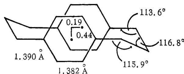
face view of crystal structure of [3.3]paracyclophane
