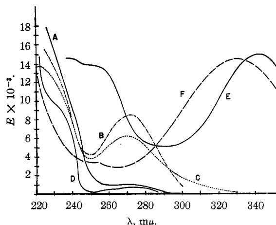
Fig. 1.—A, XII — in ethanol; B, ——— in isoöctane, by-product from cyclization of XI based on mol. wt. 290; C, I ——— in ethanol; D, XIV — in ethanol; E, — in chloroform, by-product from preparation of II, mol. wt. 595; F, ——— in ethanol-methyl 2,3,4-trimethoxybenzosuberone-6-glyoxylate.
