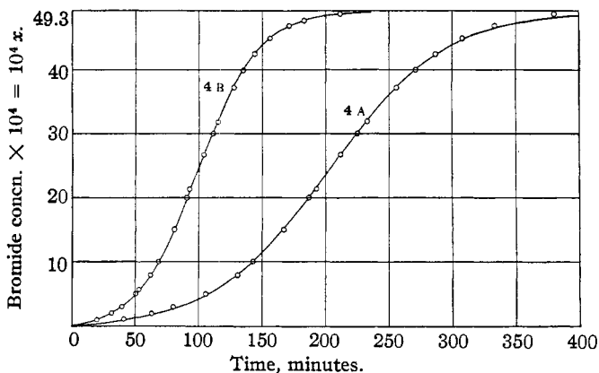
Fig. 1.—Experimental data corrected for bromide catalysis, cf. Table III. The smooth curves are calculated from Equation 13 and the constants of Table IV.
