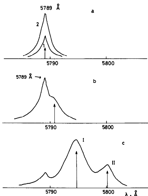
Fig. 5. The excitation spectra of ( ^5D_0 \rightarrow ^7F_1 ) luminescence in water solutions with \text{Eu}^{3+} ions in the ^7F_0 \rightarrow ^5F_0 region measured using a tunable Rhodamine 6G laser. The spectra are identical to the absorption spectra of the ^7F_0 \rightarrow ^5D_0 band. a) 1- \text{Eu}(\text{NO}_3)_3 ( 5.10^{-2} M ) in \text{H}_2\text{O} , 2- \text{Eu}(\text{NO}_3)_3 ( 5.10^{-2} M ) + \text{NaAc} ( 10^{-2} M ) in \text{H}_2\text{O} ; b) \text{Eu}(\text{NO}_3)_3 ( 5.10^{-2} M ) + \text{Phen} ( 10^{-2} M ) in \text{D}_2\text{O} ; c) \text{Eu}(\text{NO}_3)_3 ( 5.10^{-2} M ) + \text{Na}_2\text{H}_2\text{EDTA} ( 10^{-2} M ) in \text{D}_2\text{O} , \text{pD} = 5.5 , T = 295 \text{ K} .
