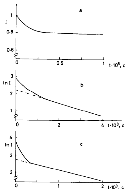
Fig. 6. The decay curves of ( ^5D_0 \rightarrow ^7F_2 ) luminescence of solutions containing \text{Eu}^{3+} solvates and one-ligand complexes \text{Eu} \cdot \text{Ac}^{2+} (a), \text{Eu} \cdot \text{Phen}^{3+} (b), \text{Eu} \cdot \text{EDTA}^- (c) after pulsed selective (advantageous) laser excitation of complexed \text{Eu}^{3+} ions only. The concentrations of solutions are the same as in Fig. 5. The wavelengths of unequilibrium excitation are shown in Fig. 5.
