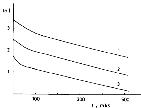
Fig. 4. The decay curves of \text{Tb}^{3+}({}^5\text{D}_4) ( 10^{-2} \text{ M} ) luminescence sensitized by an anion of salicylic acid ( 10^{-4} ) in water at 295 K and at different pH-solutions measured in total luminescence light. 1) pH = 5.7; 2) pH = 5.43; 3) pH = 5.04.
