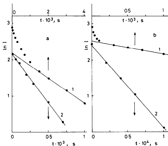
Fig. 2. The curves of intensity decay of luminescence sensitized by 1,10-phenanthroline ( 10^{-3} M ) (a) and 2,2'-bipyridine ( 10^{-3} M ) (b) of Eu^{3+} ( ^5D_0 ) ( 10^{-2} M ) in D_2O at 295 K after pulsed excitation at \lambda = 337 nm. Points denote the experimental data, straight lines represent the result of decomposition of experimental curves into two exponents; 1) Equilibrium luminescence, 2) Relaxational process.
