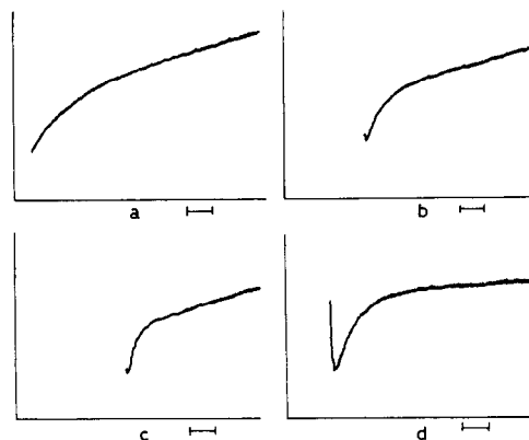
Fig. 3. Decay oscillograms of the Eu^{3+}(^5D_0) luminescence sensitized by an 1-naphthoic acid anion in methanol- d_4 (a) and in CD_3OD/D_2O mixture with D_2O 3.6% (b), D_2O 10% (c) and (d) measured in total luminescence light. The ratio of Eu^{3+} and Napht^- concentrations is 25:1. Oscillograms (a), (b) and (c) were measured with scan-speed 100 \mu s/div. , oscillogram (d) with 20 \mu s/div.
