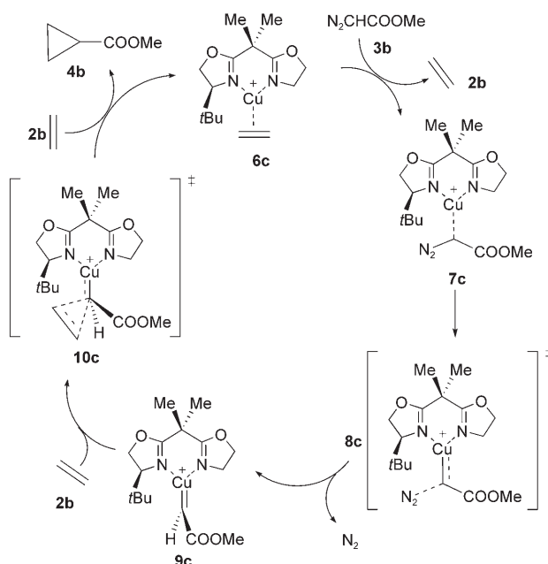
Scheme 2. Full catalytic cycle for the cyclopropanation reaction of ethylene ( 2b ) with methyl diazoacetate ( 3b ) catalyzed by the 5c –Cu I complex.
