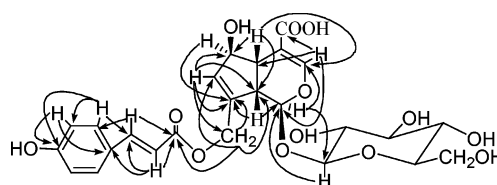
Figure 1. Selected HMBC ( \text{H} \rightarrow \text{C} ) correlations of 1 .
