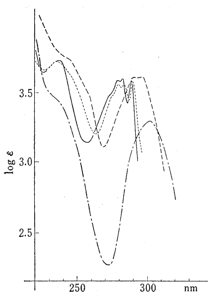
Fig. 1. UV Spectra of 1 , 2a , 3a and 4a
