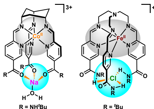
Figure 1. Differences in metal and guest binding pockets between previously reported tach- and tren-based M(II) podands. Gray and blue circles represent metal and guest binding pockets, respectively. The tach-containing pocket (left) enforces hexacoordinate geometries, while the tren-based ligand (right) allows for hexa- and hepta-coordinate geometries.
