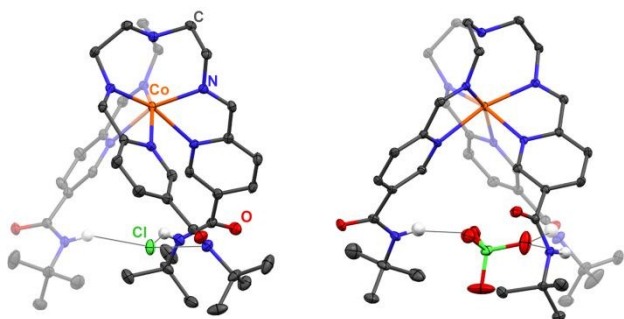
Figure 2. Crystal structures of the complex cations of 1 (left) and 4 (right) depicted with 40% thermal ellipsoids. Orange, green, red, blue, gray and white ellipsoids represent Co, Cl, O, N, C and H atoms, respectively. Hydrogen atoms not involved in hydrogen bonding and unbound anions have been omitted for clarity. The structure for 1 resides on a three-fold rotation site, while the complex for 4 sits on a general position.
