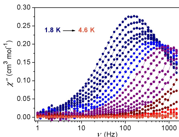
Figure 5. Variable frequency out-of-phase ac susceptibility for 1 , collected at a 2500 Oe applied dc field in the temperature range 1.8 to 4.6 K. Data were collected at 0.1 K increments from 1.8 K to 3.4 K and at 0.2 K increments from 3.6 to 4.6 K.
