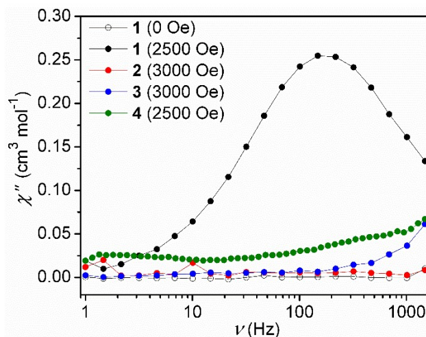
Figure 4. Frequency dependence of the out-of-phase susceptibility for 1-4 at listed applied dc fields. Data were collected at 1.9 K using a 4 Oe oscillating field. Lines are guides to the eye.
