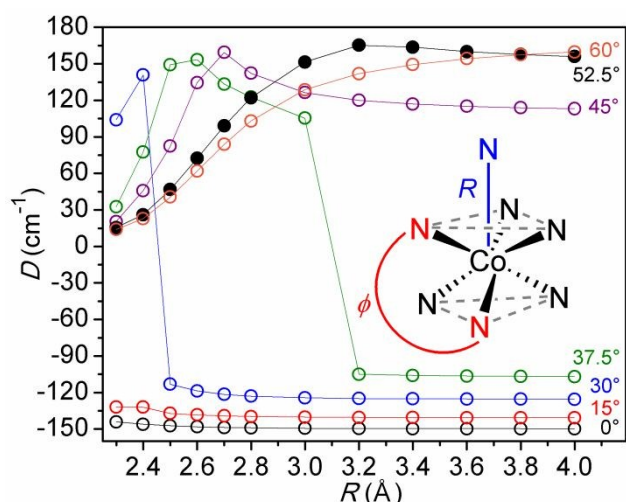
Figure 6. Calculated D values as a function of seventh Co-N distance ( R ) at given distortion angles ( \phi ), using face-capped trigonal prismatic [\text{Co}(\text{NH}_3)_7]^{2+} as a model system. The solid black data points represent the most comparable trigonal distortion to the complex salts 1-4 . Lines serve as guides for the eye.
