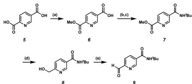
Scheme 1. Synthesis of aldehyde 9 .
