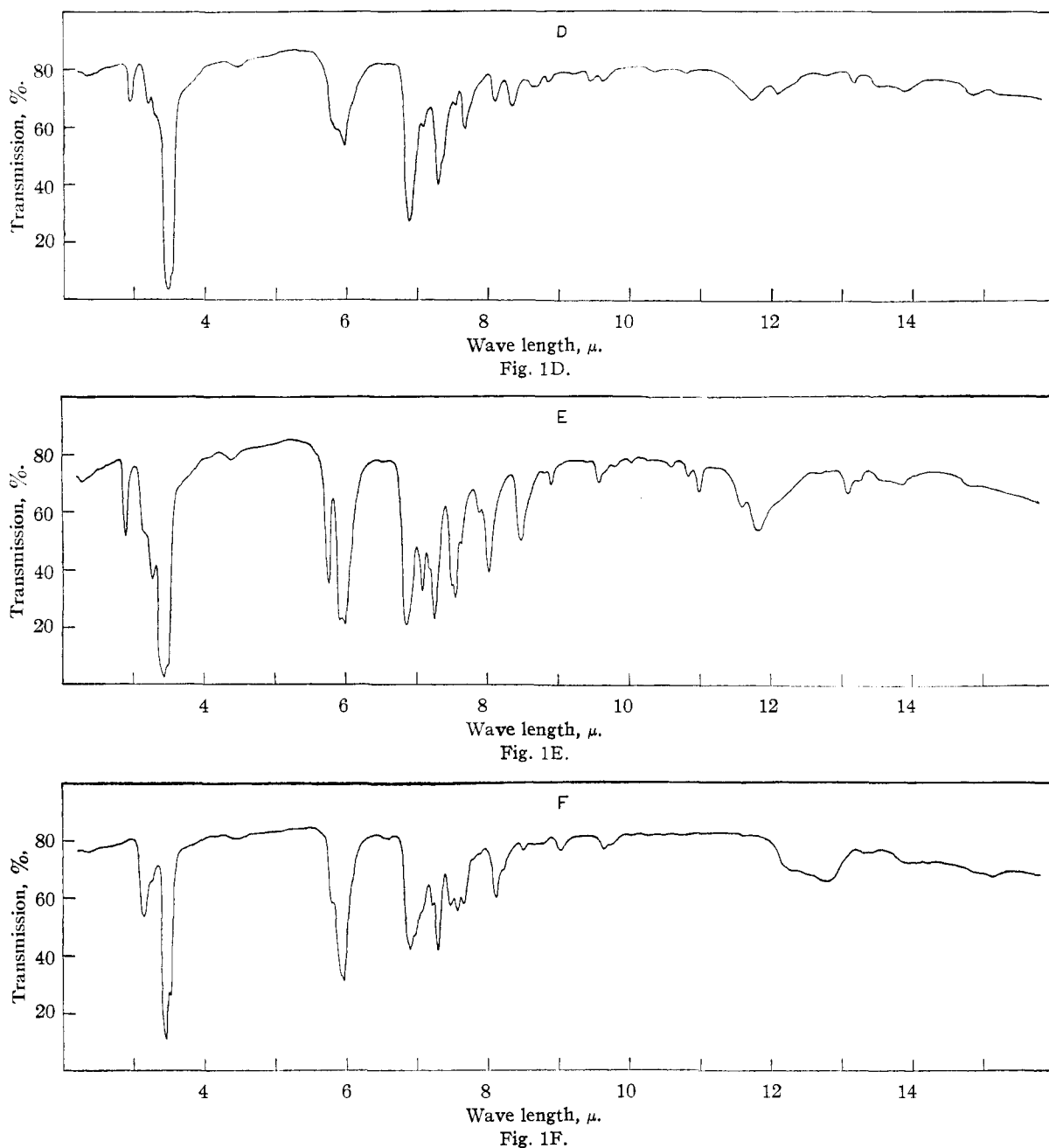
Fig. 1—Infrared absorption spectra. Measurements by R. de V. Huber, Janet Hucks and Mrs. M. P. Kraus under instruction of Dr. Harold C. Beachell. Lactone esters as pure liquids. Barbituric acid derivatives as suspensions in Nujol. A. \alpha -Carboxethyl- \alpha -ethyl- \gamma -butyrolactone. B. \alpha -Carboxethyl- \alpha -ethyl- \gamma - n -valerolactone. C. \alpha -Carboxethyl- \alpha -ethyl- \gamma -isocapro lactone. D. 5-Ethyl-5-( \beta -hydroxypropyl)barbituric acid. E. 5-Ethyl-5-( \beta -hydroxyisobutyl)barbituric acid. F. 5-Ethyl-5-( \beta -chloroisobutyl)barbituric acid.
