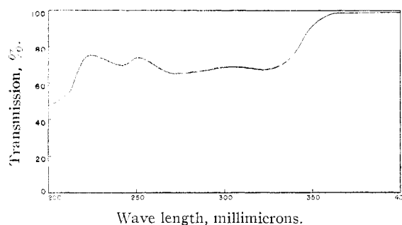
Fig. 2.—Ultraviolet absorption spectrum of unidentified compound obtained from the reaction of isoquinoline with hexafluorocyclobutene ( C_2H_4N_2OF_4 ), c , 1.01 \times 10^{-5} mole/liter.
