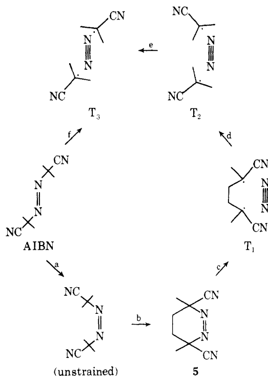
Scheme 1. Thermochemical Cycle for a Six-Membered Azoalkane
