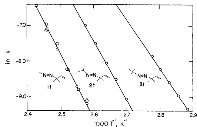
Figure 1. Arrhenius plot for trans azoalkanes. k is in sec –1 . (O) Gas evolution in p -diisopropylbenzene; (Δ) gas evolution in 0.26 M benzoquinone in diphenyl ether; (□) NMR in p -diisopropylbenzene.
