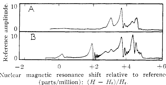
Fig. 1.—Nuclear magnetic resonance spectra: curve A, \psi -santonin acetate; curve B, methyl 1-keto-7-acetoxy- \Delta^{5(10)} -santenate. The following operating conditions were employed: frequency, 30 mc.; sweep width, 56 milligauss; sweep rate, 5.6 mg./sec.; H_1 amplitude, 3.5-low; reference, H_2O .
