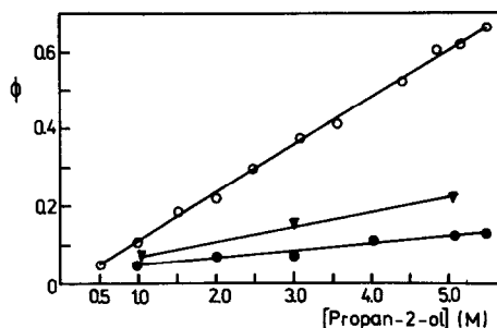
Fig. 1. \phi_{Co^{2+}} , \phi_{Cr(VI)} , \phi_{Cr(VI)} in absence of cobalt-(III) vs. concentration of propan-2-ol in 10^{-5} M H^+ solutions. [K_2CrO_4] and [Co(NH_3)_5H_2O](ClO_4)_3] = 10^{-3} M .
