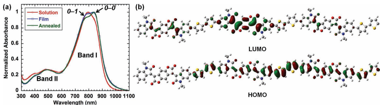
Figure 1. a) Normalized absorption spectra of BDOPV-2T in \text{CHCl}_3 ( 1 \times 10^{-5} \text{ M} ), thin film, and annealed film ( 200^\circ\text{C} for 5 min). b) Calculated molecular orbitals of the trimer of BDOPV-2T (B3LYP/6-311G(d,p)).
