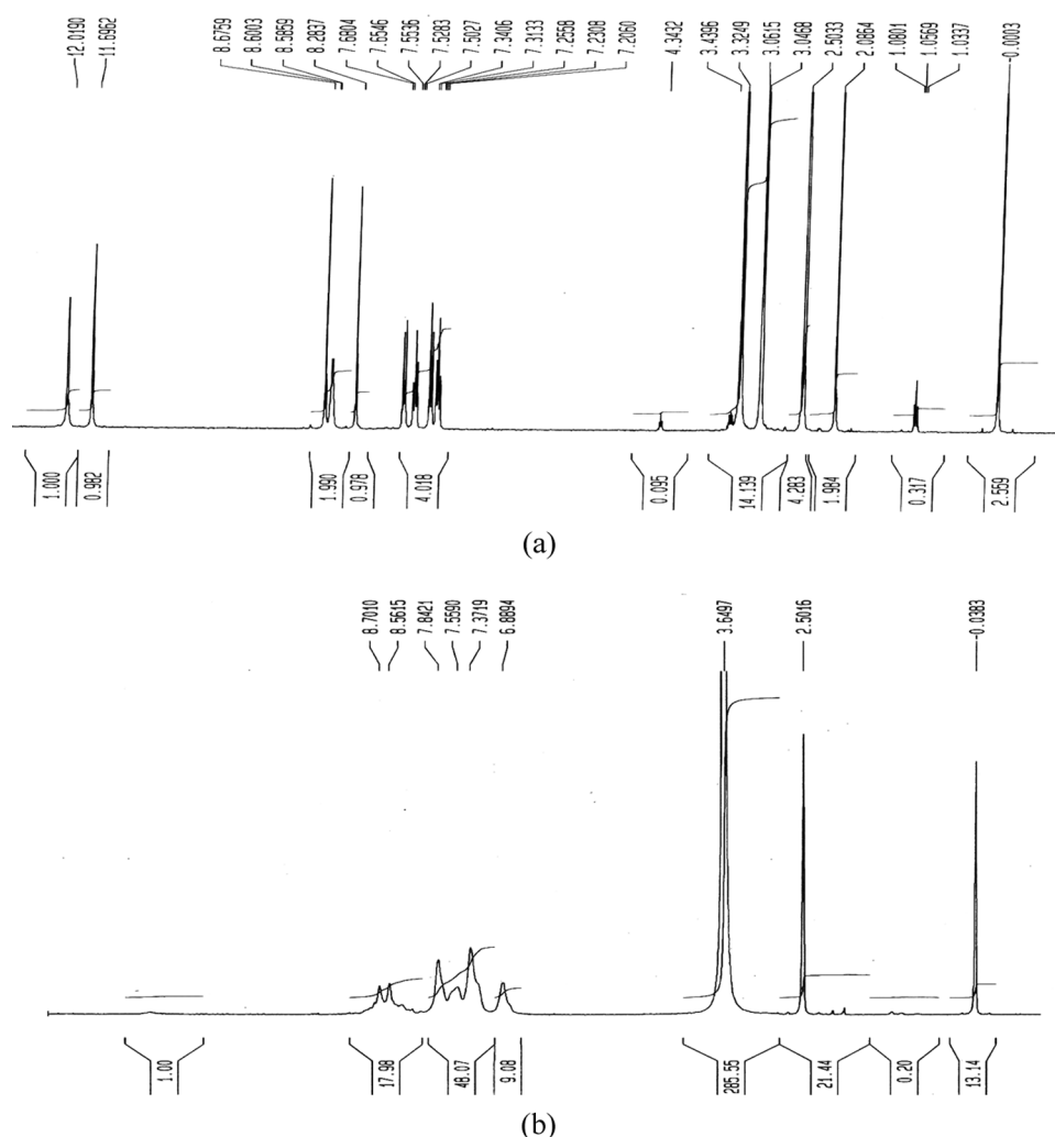
FIGURE 1 ^1\text{H} NMR spectra. (a) ^1\text{H} spectrum of L 1 H 2 . (b) ^1\text{H} spectrum of L 1 HZN.
